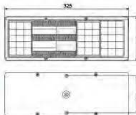
LED- 瑞琪后尾灯 LED TAIL LAMP
