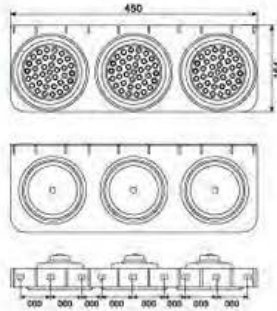
LED- 中集橡胶后尾灯 (三体) LED TAIL LAMP
