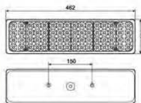
LED- 斯太尔王超薄铁制后尾灯 LED TAIL LAMP
