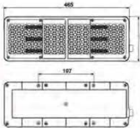
LED- 新型悍威、加宽奥威后尾灯 LED TAIL LAMP
