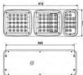
LED- 巨能王后尾灯 (七彩) LED TAIL LAMP
