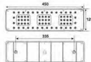
LED- 豪沃多功能后尾灯 LED TAIL LAMP
