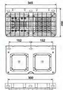
LED-153 箭头加七彩后尾灯 LED TAIL LAMP
