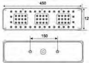
LED- 斯太尔王多功能后尾灯 LED TAIL LAMP
