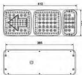
LED- 巨能王后尾灯 (箭头) LED TAIL LAMP
