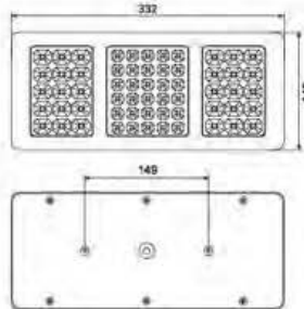
LED- 仿斯太尔后尾灯 LED TAIL LAMP
