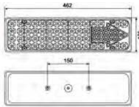
LED- 斯太尔王后尾灯 (箭头) LED TAIL LAMP
