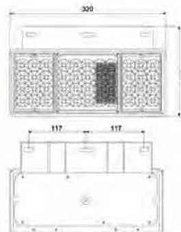
LED- 塑制 - 五十铃后尾灯 LED TAIL LAMP
