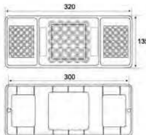
LED- 东风 140-2 塑制防水型后尾灯 LED TAIL LAMP
