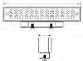
LED- 边灯 LED SIDE LAMP
