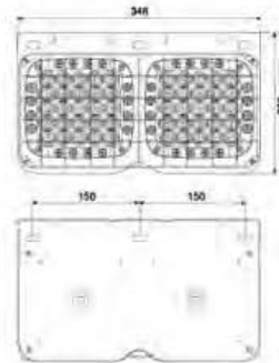
LED-153 铁制七彩后尾灯 LED TAIL LAMP
