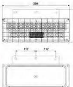
LED-江淮 808 后尾灯-黑 LED TAIL LAMP
