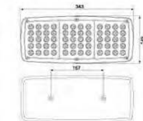
LED- 老斯太尔后尾灯 (多管) LED TAIL LAMP
