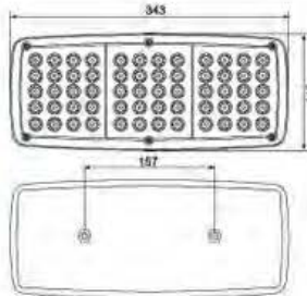
LED- 老斯太尔后尾灯 (多管) LED TAIL LAMP
