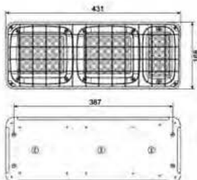
LED- 巨能王铁制后尾灯 (封闭式防水型带网罩) LED TAIL LAMP
