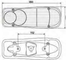
LED- 东风紫罗兰后尾灯 LED TAIL LAMP
