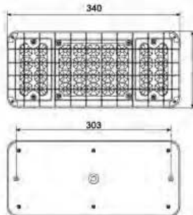
LED- 东风 140-2 铁制后尾灯 LED TAIL LAMP
