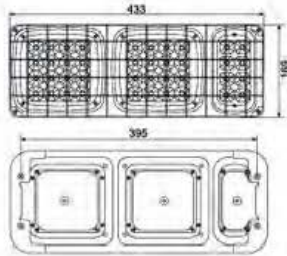
LED- 巨能王铁制后尾灯 LED TAIL LAMP
