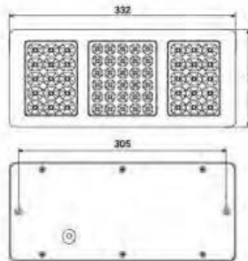
LED- 东风 140-2 后尾灯Ⅲ型 LED TAIL LAMP
