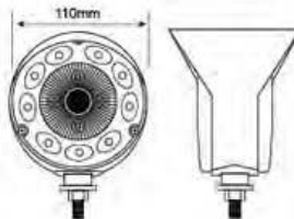
LED- 后尾灯 LED TAIL LAMP
