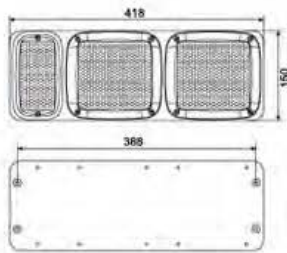
LED- 巨能王铁制后尾灯 (防水型) LED TAIL LAMP
