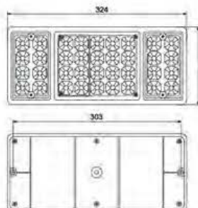
LED- 东风 140-2 后尾灯 (七彩) LED TAIL LAMP
