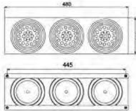
LED- 中集橡胶后尾灯 (三体) LED TAIL LAMP
