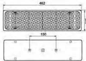
LED- 斯太尔王铁制后尾灯 (加厚) LED TAIL LAMP
