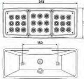
LED- 老斯太尔后尾灯 LED TAIL LAMP
