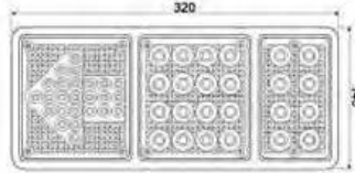
LED- 边灯 LED SIDE LAMP
