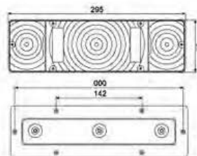
LED-131 后尾灯 LED TAIL LAMP
