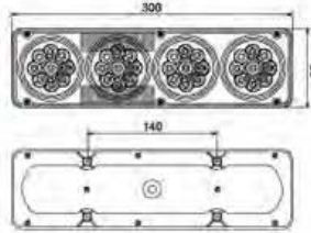
LED-588 小金刚后尾灯 LED TAIL LAMP
