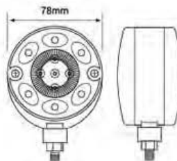
LED- 后尾灯 LED TAIL LAMP
