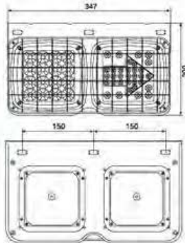
LED-153 后尾灯 (箭头) LED TAIL LAMP
