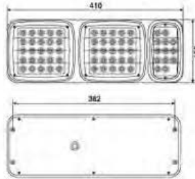
LED- 巨能王后尾灯Ⅳ型 LED TAIL LAMP
