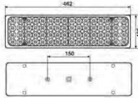
LED- 斯太尔王后尾灯 (塑) LED TAIL LAMP
