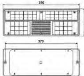
LED- 江淮后尾灯 ( 塑制 ) LED TAIL LAMP
