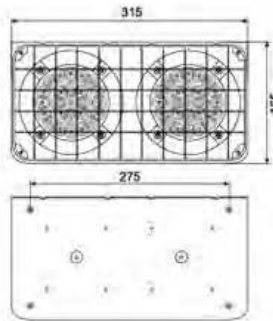
LED- 高亮中集铁制后尾灯 (封闭式防水型, 带网罩) LED TAIL LAMP
