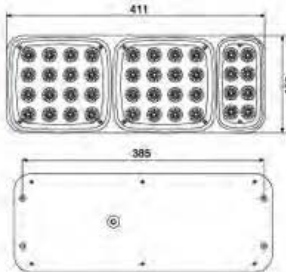
LED- 巨能王后尾灯Ⅲ型 LED TAIL LAMP
